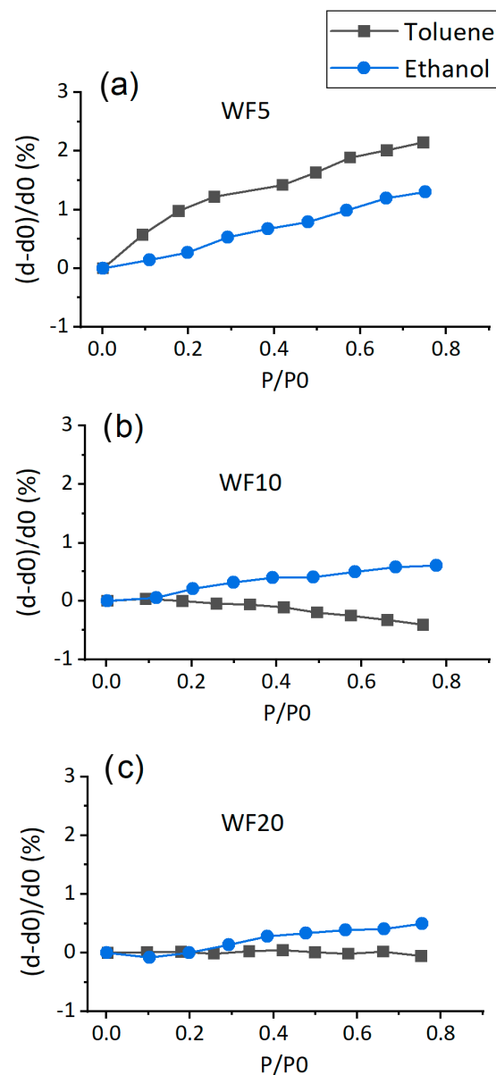
Figure 5. Swelling of the elaborated PP-HMDSO thin films while exposed to toluene or ethanol atmospheres, P_0 being the saturated vapor pressure. d_0 is the initial film thickness under vacuum and d is its thickness under P/P_0 of toluene or ethanol. (a) WF5, (b) WF10 and (c) WF20.
