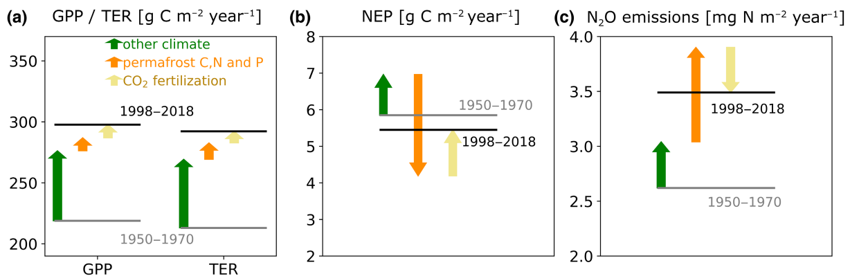
FIGURE 9 Simulated response of Gross primary productivity (GPP) and total ecosystem respiration (TER, panel a), net ecosystem production (NEP, panel b) and N 2 O emissions (panel c) to climate effects other than increased permafrost nutrients and carbon (other climate, green), permafrost C, N, and P (orange) and CO 2 fertilization (khaki), all averaged over all sites.
