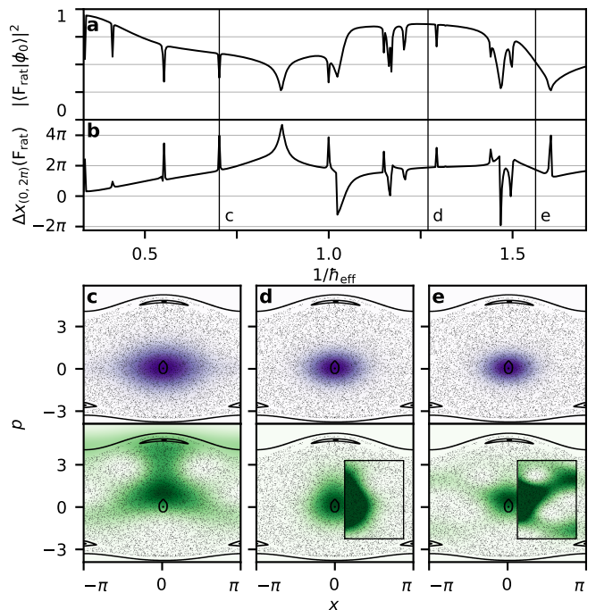
FIG. 2. Eigenstate and transport dependences on the effective Planck constant. (a) Overlap between the ground state |\phi_0\rangle of the lattice and the ratcheting Floquet state |\text{F}_{\text{rat}}\rangle and (b) transport (2) of |\text{F}_{\text{rat}}\rangle over one modulation period as a function of 1/\hbar_{\text{eff}} . (c-e) Stroboscopic phase portraits in the unit cell of system (1) and Husimi representations of |\phi_0\rangle (top, purple) and |\text{F}_{\text{rat}}\rangle (bottom, green) for the values of 1/\hbar_{\text{eff}} = 0.70, 1.27, 1.56 respectively, identified by vertical lines on the panels (a-b). The color range for each Husimi function extends from zero to its maximum value, with a truncation from a quarter of this value in the outlined rectangular regions of panels (d,e) in order to reveal details (note that the Floquet states share the x \rightarrow -x symmetry of the phase portrait).
