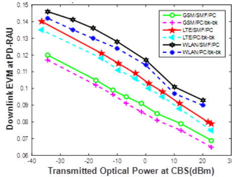
Figure 4. Comparison of the multiservice OCDM-PC of operator-1
