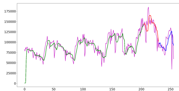
Fig. 7. Forecasting curves of Transformers model for Colecalciferol
