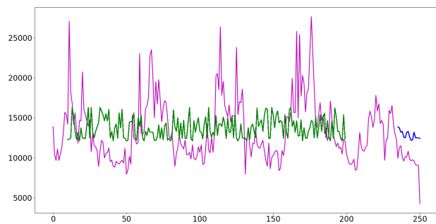
Fig. 6. Forecasting curves of LightGBM model for Cetirizine
