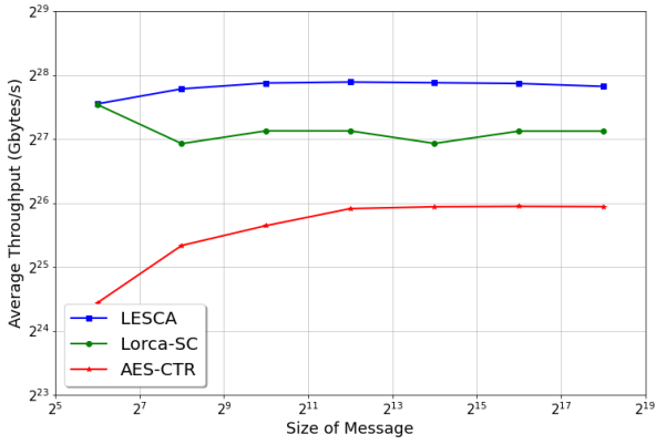
(c) RPI3
