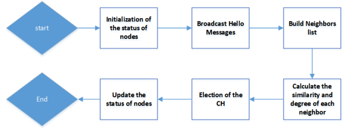
Fig. 2. Proposed Clustering Algorithm Flowchart
