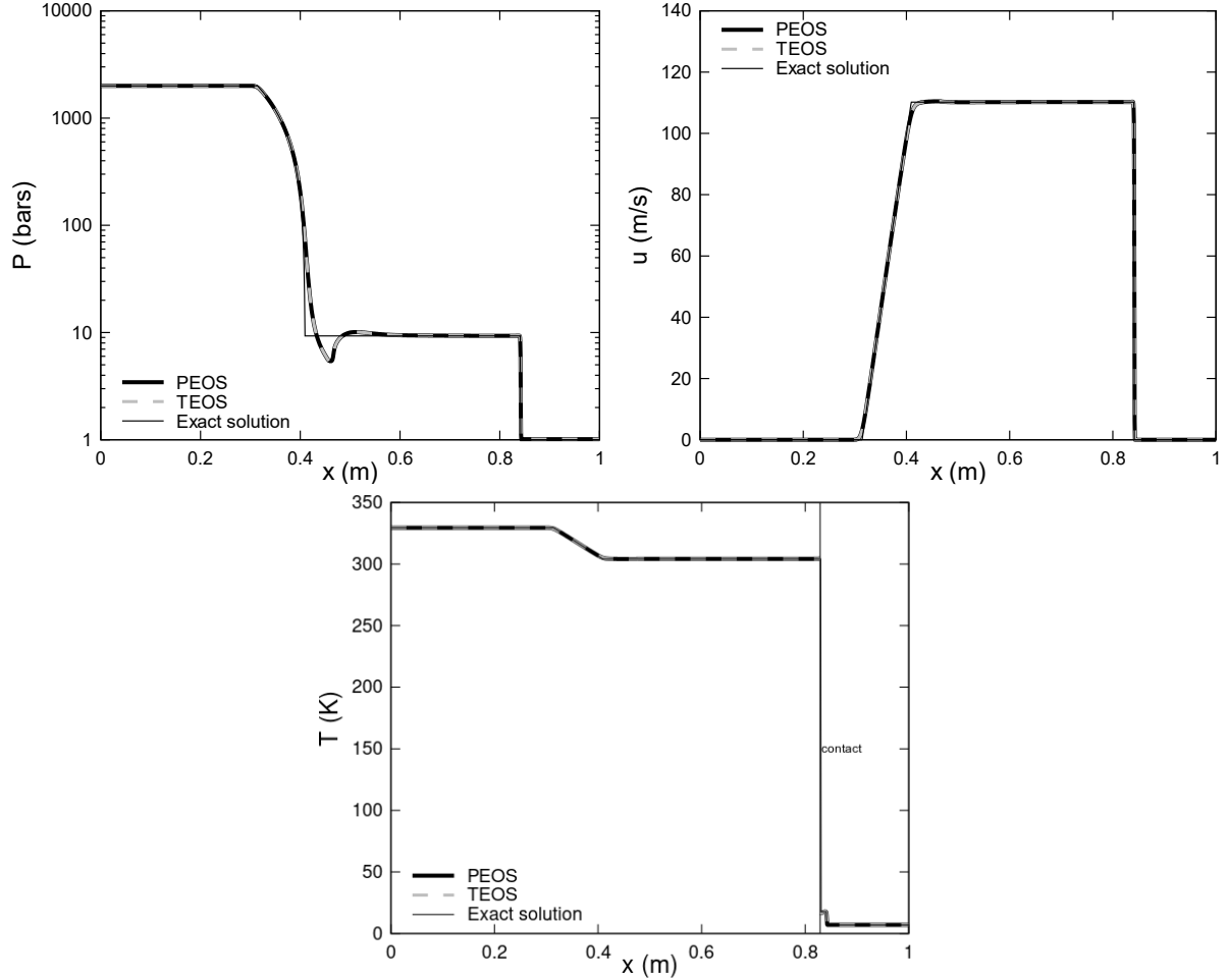
Figure 8. Shock-tube test case with the symmetric variant of the Baer and Nunziato equations with instantaneous velocity and pressure relaxations. Dashed gray lines represent computed results with the conventional method (TEOS), and black lines correspond to the relaxation method (PEOS). Thin black lines represent the exact solution computed with the Riemann solver of Saurel et al. (1994). Results are shown at time 276 \mu\text{s} . As pressure and velocity are instantaneously relaxed, only one pressure and one velocity are displayed. Since temperatures are in disequilibrium, the nitromethane temperature is shown on the left of the contact, while the air temperature is displayed on the right. The present relaxation method perfectly recovers the target EOS results.
