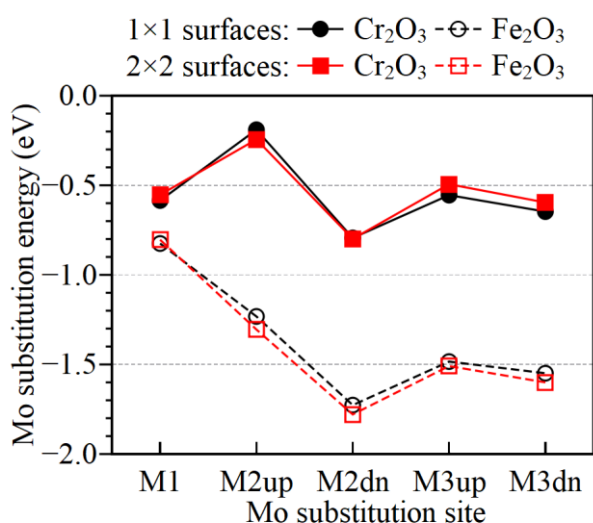
Figure 5. Mo substitution energy from terminating “M1” site in the topmost layer to “M3dn” site in the 3 rd metal layer calculated with 1 \times 1 and 2 \times 2 \text{Cr}_2\text{O}_3 and \text{Fe}_2\text{O}_3 (0001) surface cells.
