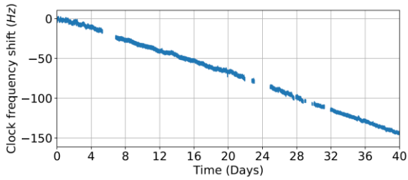
Figure 1: Temporal trace of the clock frequency for a Cs-He cell with BSG windows.
