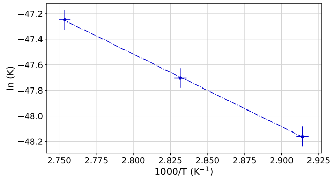
FIG. 5. Permeation constant K (logarithm) versus the inverse of the cell temperature T ( 1000/T ), for an ASG-based cell.
