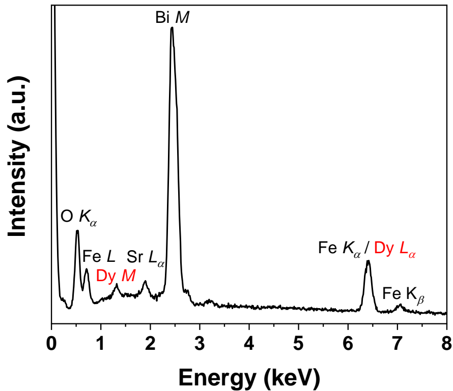
Figure S2. EDX spectrum of a BDFO 8% film.
