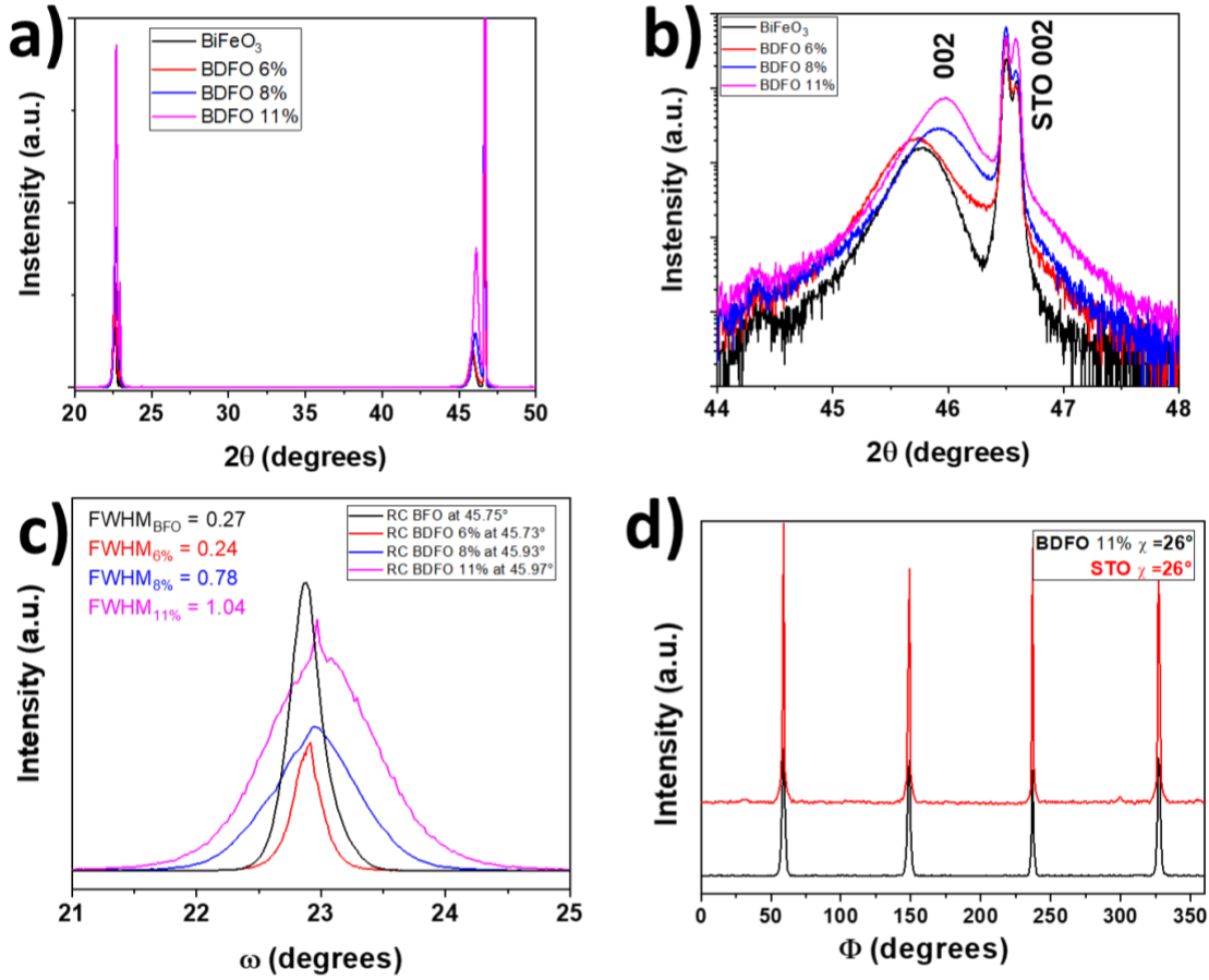
Figure 1 XRD patterns of the doped and undoped BFO films: a) \theta - 2\theta patterns and b) enlarged 2\theta region in the 44^\circ - 48^\circ ; c) rocking curves of the BFO and BDFO films around their 002 reflections; d) \phi scan of 210 reflections of the BDFO 11% film and the STO:Nb substrate.
