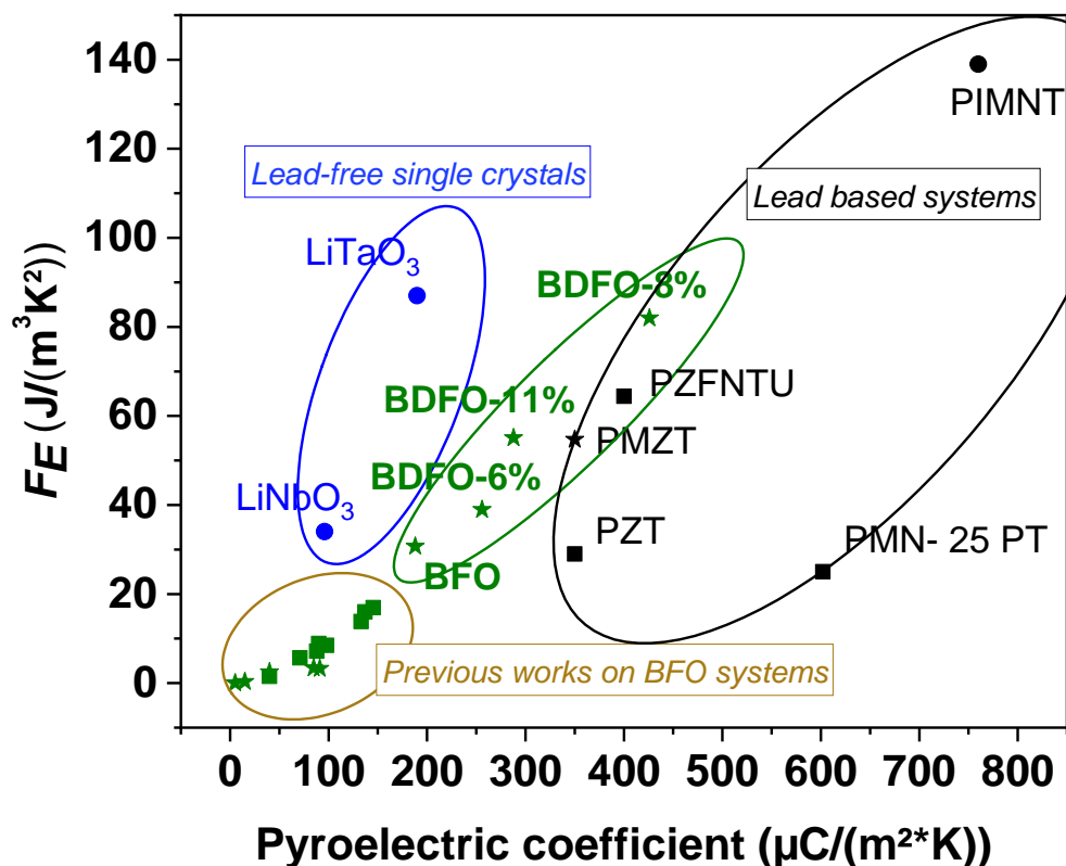
Figure 9. Comparison between pyroelectric coefficients and F_E obtained in this work (green stars grouped in the green circle) and previous values of BFO related systems in film form (green stars) and ceramics (green squares); lead based systems in film form (black star), ceramics (black square) and single crystal (black circle); and lead-free single crystals (blue circle).
