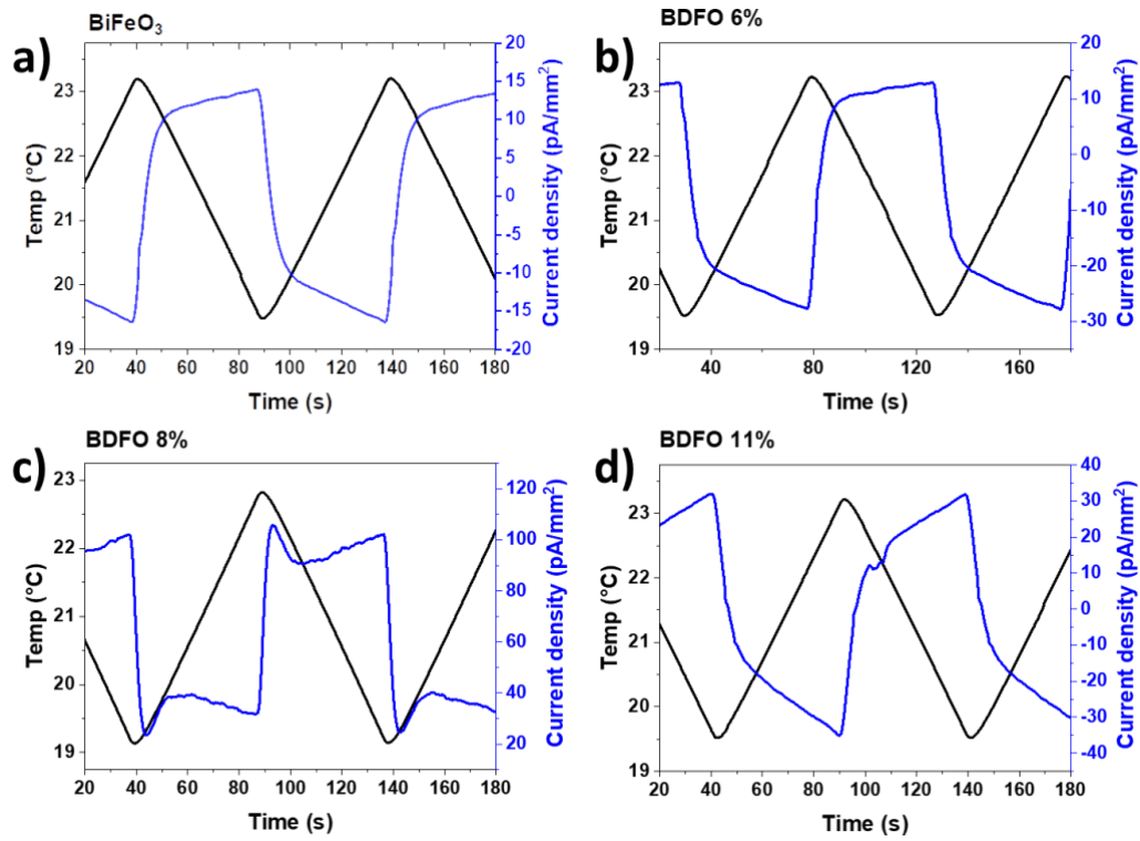
Figure S4. Single cycle pyroelectric responses of a) BiFeO 3 , b) BDFO-6%, c) BDFO-8% and d) BDFO-11% thin films to a triangular temperature waveform \Delta T=4^{\circ}\text{C} at RT.
