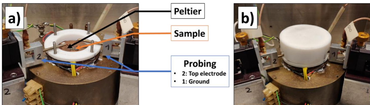
Figure S3. a) Insertion of the sample to measure the pyroelectric current. The sample is in contact with the Peltier element and is probe between the top Au/Cr electrode and bottom STO:Nb conductive substrate and b) To avoid external thermal gradient, the sample is brought to equilibrium temperature and pre-cycled to avoid thermally stimulated current.
