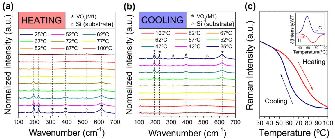
Figure 6. Raman spectra recorded for sample T200_550_45 at multiple temperatures between 25 and 100°C during consecutive (a) heating and (b) cooling cycles. (c) Thermal evolution of the intensity of the VO 2 (M) Raman band at 194 cm -1 during heating (red) and cooling (blue) cycles. The inset shows the derivative of each kinetic thermochromic cycle (the derivative of the cooling is plotted in absolute values).
