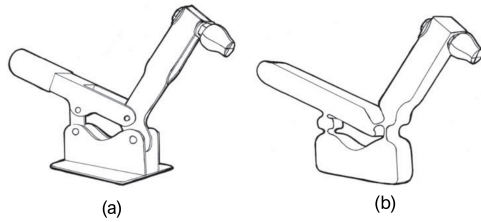
Fig. 2. Mechanisms, (a) rigid-body mechanism of a hold-down clamp (18 parts), (b) compliant hold-down clamp concept (1 part). [51]
