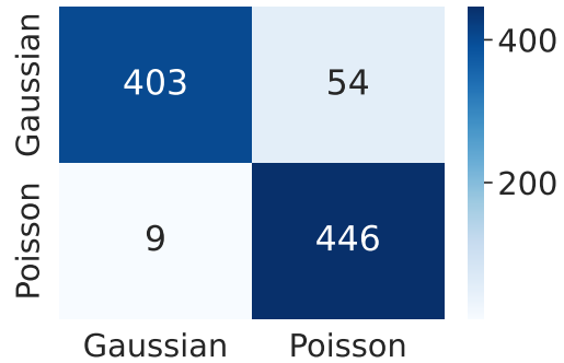
Figure 3. Confusion Matrix.
