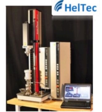
Axial testing
