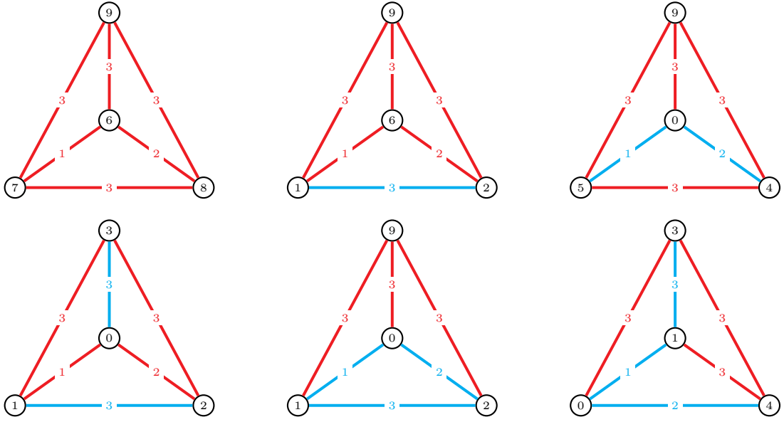
Figure 4: Abs-proper 3-labellings of all canonical signatures of K_4 . In each picture, positive and negative edges are represented as red and blue edges. In each vertex the resulting absolute sum is indicated by the depicted labelling.
