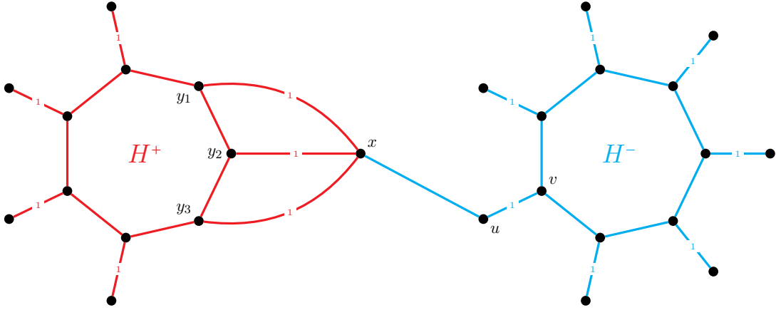
Figure 2: Illustration of the construction of G in the proof of Theorem 2.9, given together with a partial proper 2-labelling. Positive and negative edges are represented as red and blue edges.
