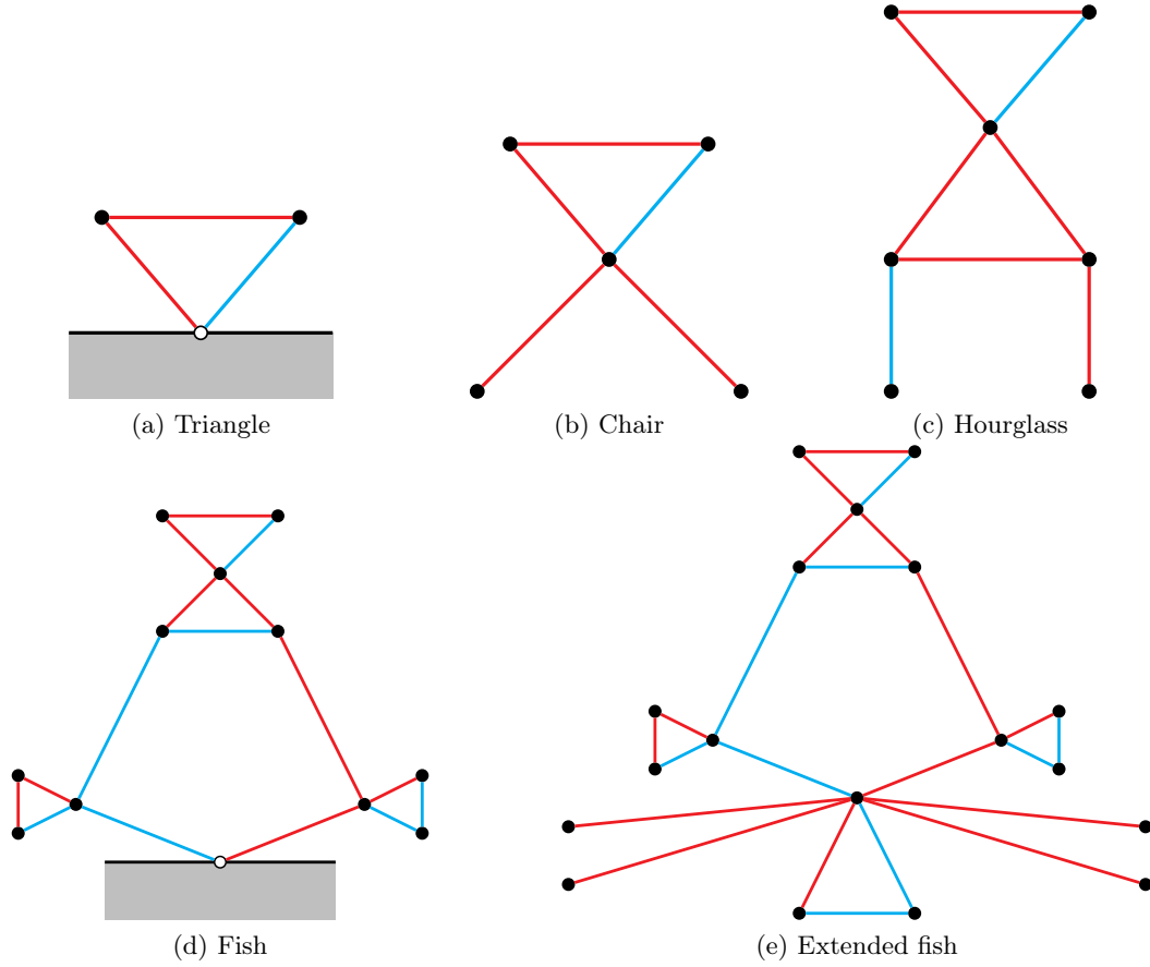
Figure 5: Constructions and gadgets used in the proof of Theorem 5.6, together with (part of) a possible locally irregular signature. In attaching constructions, the structure is attached at the white vertex, with the original graph represented by the gray area. In each picture, positive and negative edges are represented as red and blue edges.
