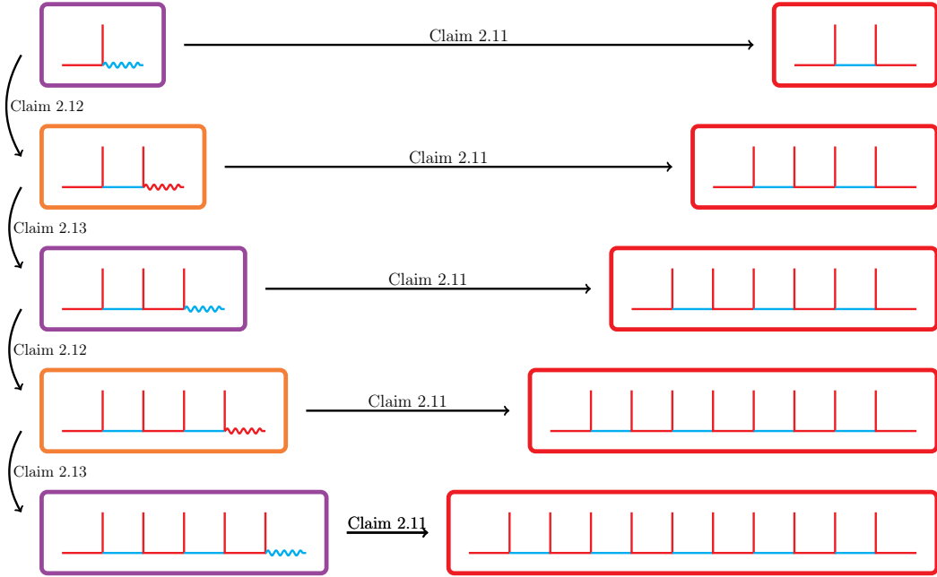
Figure 3: First steps of the construction of arbitrarily large signed trees with no abs-proper 2-labellings, described in the proof of Theorem 2.10. Any arrow joining two trees indicates which construction, from Claims 2.11 to 2.13, is applied. Signed trees in purple and orange boxes are intermediate pieces, while signed trees in red boxes have the desired property. Wiggly edges in purple boxes are \alpha -forced edges, while those in orange boxes are \beta -forced edges. Positive and negative edges are represented as red and blue edges.
