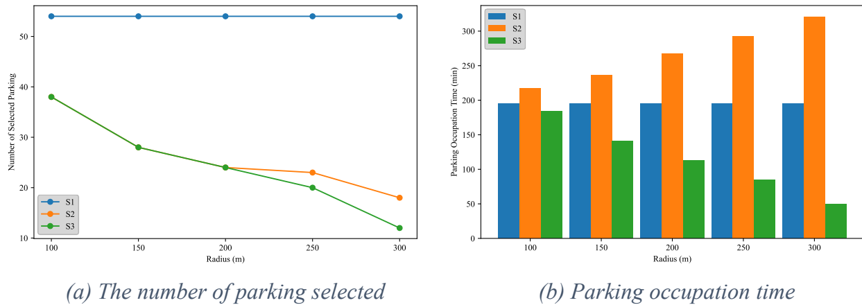
Figure 9. Parking demand and the use time (the constant value of S1 is for illustrative and benchmarking purposes and has no correlation with the catchment radii).
