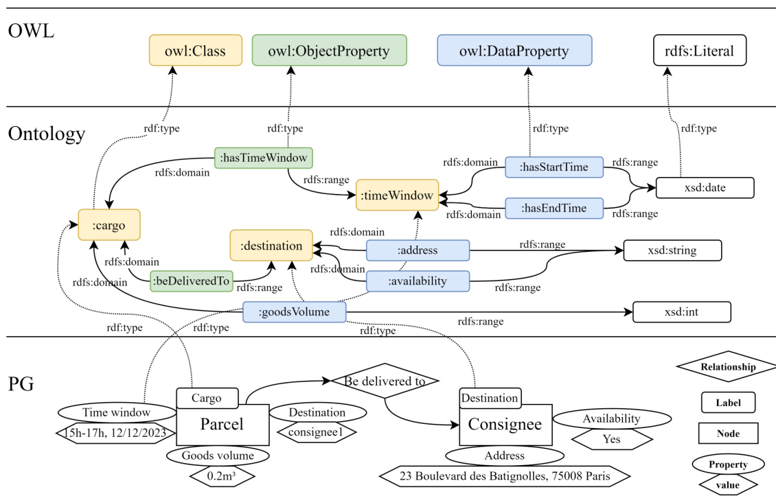
Figure 2. An example of PG-stored DT-related data abstracted into ontology with OWL.
