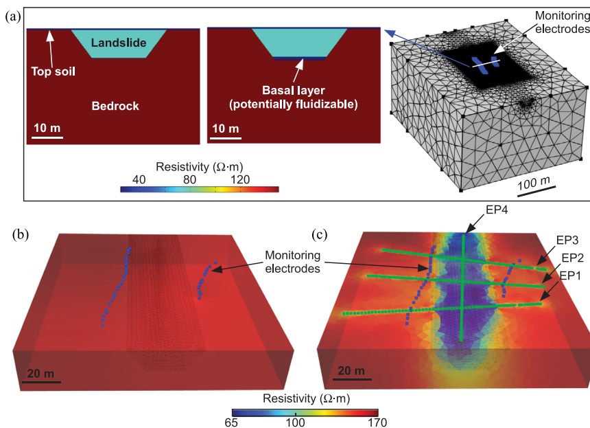
Figure 5 Numerical study. (a) Computation domain. (b) Inversion result without a starting model. (c) Inversion result using a starting model.
