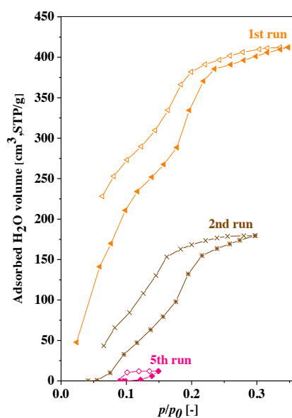
34 35 Figure 4. Effect of repeated H 2 O uptake measurements at 20 °C on the same sample, each 36 cycle being followed by re-evacuation (without heat treatment or removal from the sample 37 port) at 20 °C. All water uptakes are normalized with respect to water-free mass. 38 39
