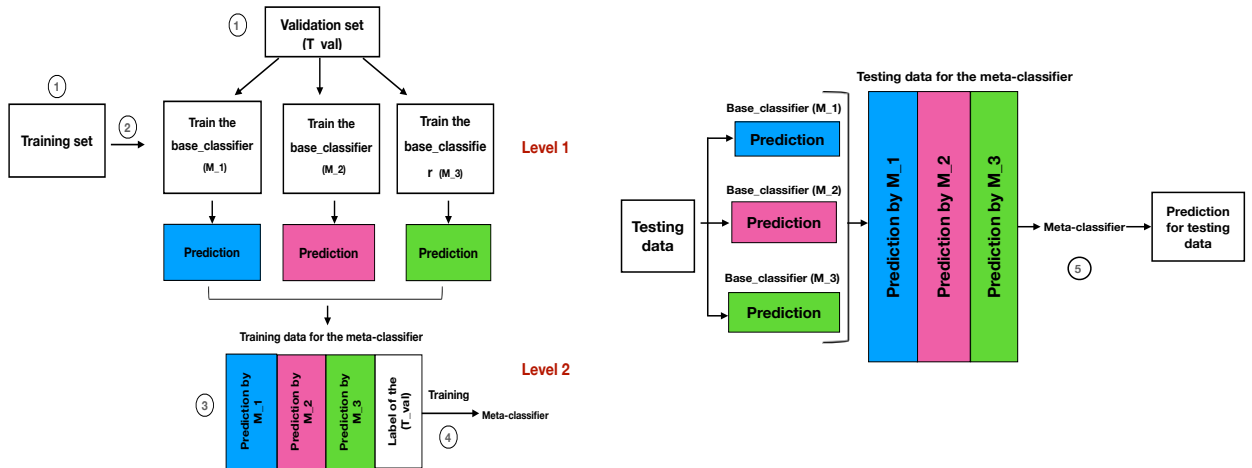
Figure 1: Training process (left) and Test process (right)
