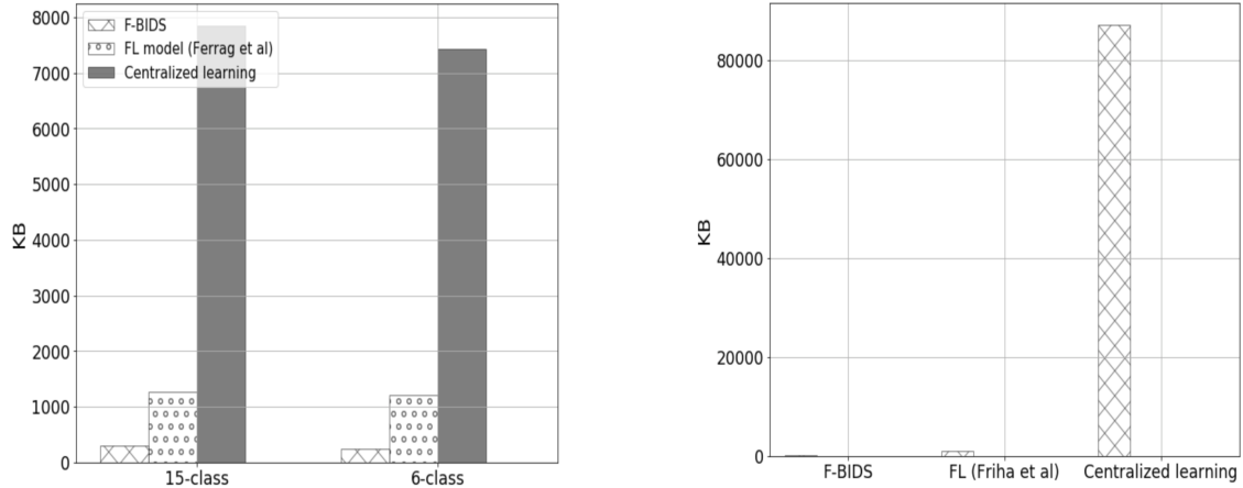
Figure 5: Communication overhead with Edge_IIoT dataset (left) and for InSDN dataset (right)
