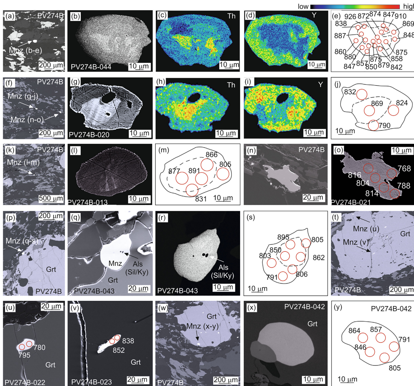
Fig. 9. Backscattered electron (BSE) images and compositional maps of representative monazite grains from Grt-Sil-Ky gneiss PV274B. Shown are monazite textural positions, close-up BSE images with analytical number of the monazite grain, Th- and Y-compositional maps and sketches with analytical points (10 \mu\text{m} ) and resulting dates. (a–o) Matrix monazite; (p–y) Monazite included in garnet. For details see text.
