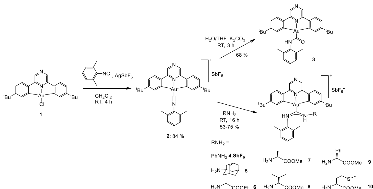
Scheme 1 Synthesis of (\text{C}^{\wedge}\text{N}^{\text{pz}}\wedge\text{C})\text{Au} complexes 2-10 .
