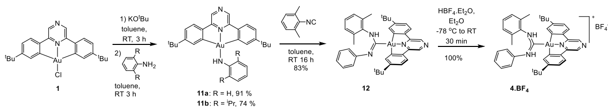
Scheme 2 Synthesis of acyclic carbene 4 · \text{BF}_4^- from gold(III) anilide.
