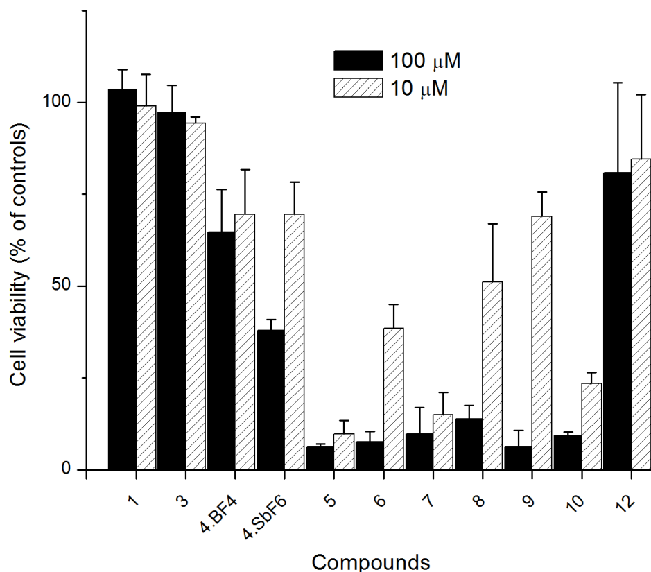
Fig. 4 Inhibition of A549 cells growth by complexes 1 , 3 - 10 and 12 in DMSO; data represent the average \pm standard error of three experiments.
