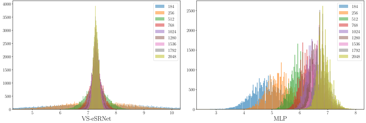
Figure 9: Histograms of the VS-eSRNet’s and MLP’s logits for cover images of size N \times N .
