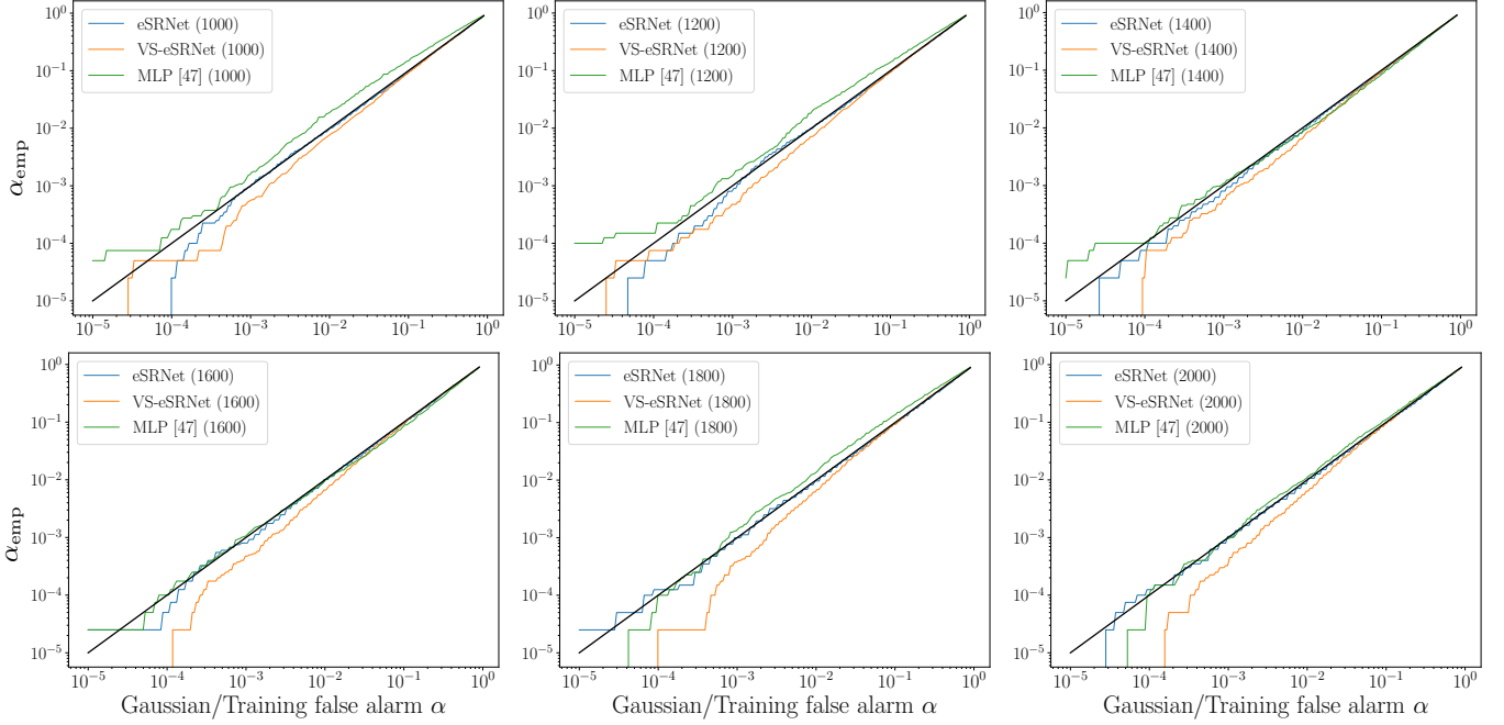
Figure 8: Comparisons between prescribed FPR \alpha and practical FPR \alpha_{\text{emp}} for the different schemes and images of sizes N \times N ( N is listed in the legend). The MLP’s \alpha_{\text{emp}} is shown as a function of the empirical FP rate on its training images of the closest size in \mathcal{S}_{\text{train}} .
