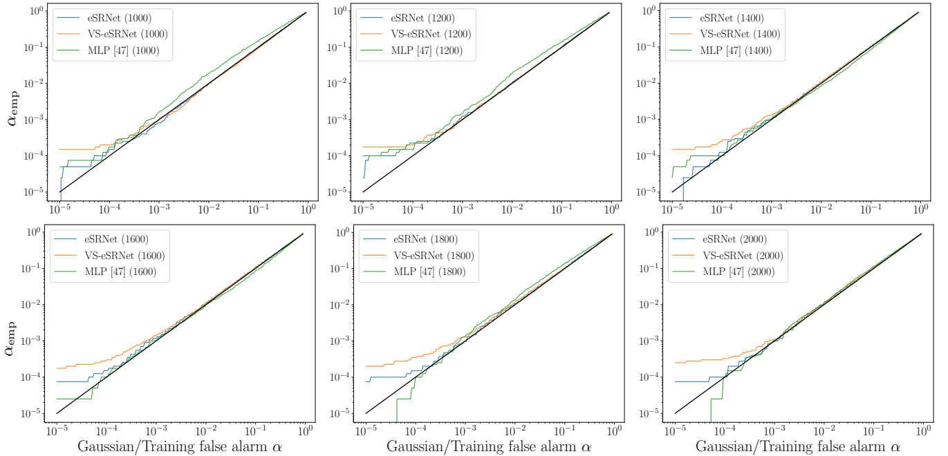
Figure 8: Comparisons between prescribed and practical FPR for the different schemes. for images of sizes N \times N . The MLP’s \alpha_{\text{emp}} is shown as a function of the FP rate on training images of the closest size in \mathcal{S}_{\text{train}} .
