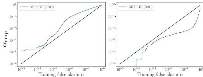
Figure 10: The MLP’s \alpha_{\text{emp}} as a function of the FP rate on insufficient training images of the closest size in \mathcal{S}_{\text{train}}^{(1)} and \mathcal{S}_{\text{train}}^{(2)} .
