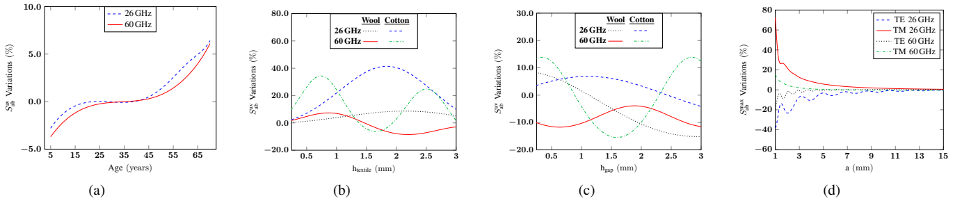
Figure 2: Variations of the S_{ab} with respect to the case of a planar homogeneous skin model (a) as a function of age, (b) textile thickness, (c) air gap thickness in presence of a textile, and (d) body curvature radius.
