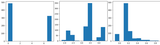
Figure 2: Histograms of the minimum of all costs appearing on the diagonal of each learned cost matrix for constrained pairs of cells (i.e., on the same row, column or sub-square) using the regular NPLL (left), the E-NPLL with k=10 (middle) and the Hinge loss (right). In the Sudoku rules, all these costs are infinite in order to prevent 2 constrained cells to contain the same value. In these histograms, a positive cost shows that a constraint has been learned. The NPLL missed many constraints, implying many rules have not been learned. The E-NPLL learns all 810 constraints, i.e., exactly the expected rules, while the Hinge loss omits some redundant constraints (preserving 100% accuracy).
