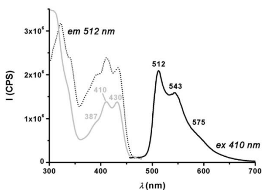
Figure 3. Emission (black solid line) and excitation (black dotted line) bands of (C N ^p z ^C)AuH ( AuH ) in PMMA (10 wt-%), and UV-Vis absorption spectrum (grey line) of AuH in CH 2 Cl 2 ( 10^{-5} M) at 298 K.
