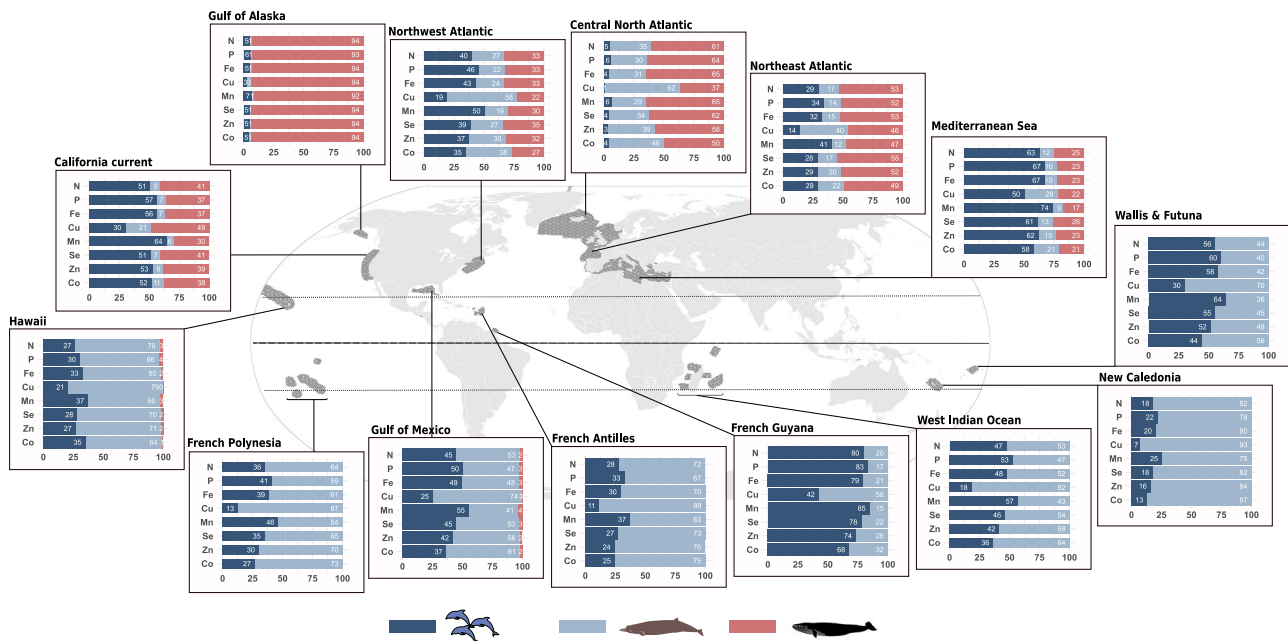
Fig. 6 | Different cetacean taxa show different contributions to nutrient cycling worldwide. Respective contribution (in %) of baleen whales (red), deep divers (light blue) and small cetaceans (dark blue) to loads of nutrients released by whole cetacean communities in 14 contrasted areas. Results are from the bioenergetic model supplemented with an original dataset of abundance estimates, diet
