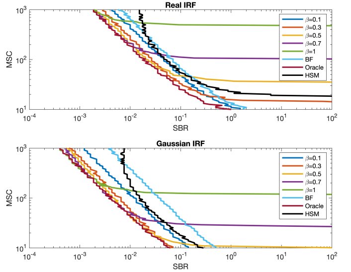
Fig. 2: Curves of satisfactory detection ( p_d = 85\% , with \eta = 28 ) as a function of the SBR and mean signal count (MSC) using the real IRF (top) and Gaussian IRF (bottom). This figure compares HSM and (pseudo-)MMSE estimators using the same Gaussian prior distribution with mean 600 and variance 2500.
