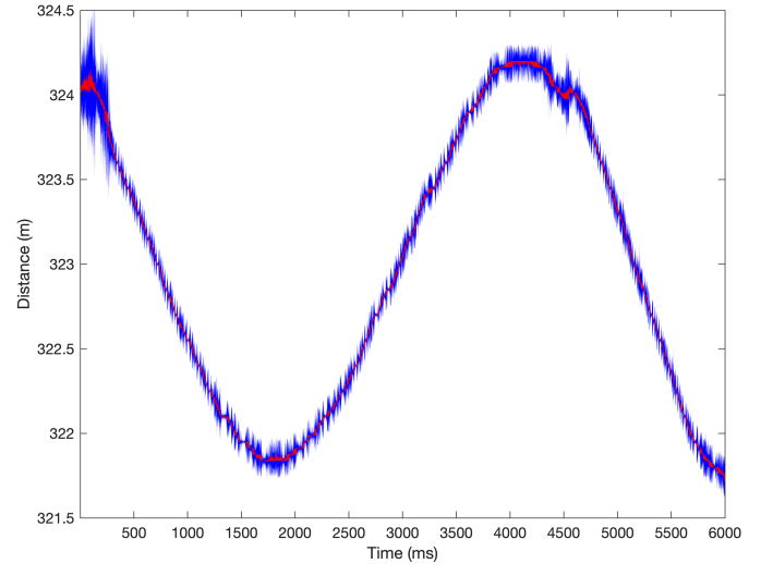
Fig. 5: Temporal evolution of the estimated depth in pixel (16,16) of the second experiment (running pedestrian). The red curve represents the mean of the depth posterior distribution obtained for each frame and the blue region represents the \pm 6 standard deviation credible interval.
