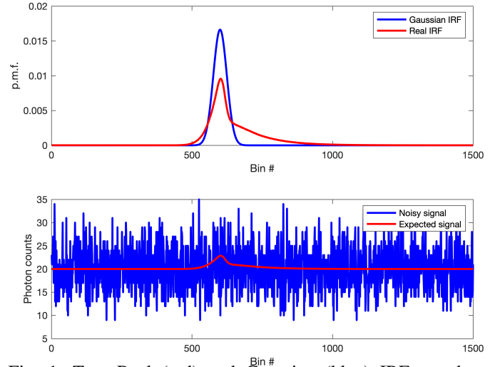
Fig. 1: Top: Real (red) and Gaussian (blue) IRFs used to simulate synthetic data. The position of the peak is bin 600 for each IRF. Bottom: Example of expected (red) and noisy (blue) histogram of photon counts, using the real IRF, for 300 signal photons and \text{SBR} = 10^{-2} (the peak is located at bin 600).
