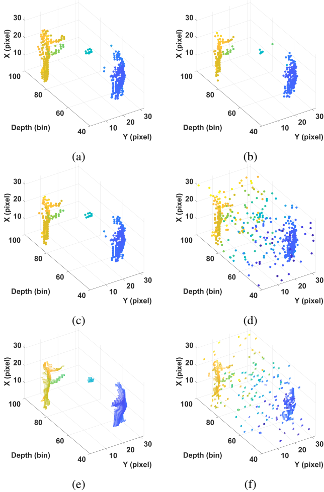
Fig. 4: Examples of 3D reconstruction using the proposed method ((a),(b)), BF ((c),(d)) and RT3D (e),(f). The left-hand side plots correspond to actual measurements while the right-hand side plots have been obtained from the pseudo-synthetic data generated with additional background ( b = 50 ). The colormap represents the surface depth (axial direction).
