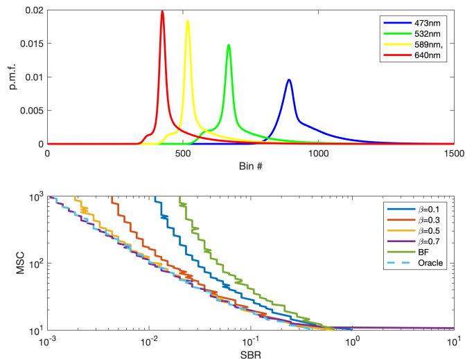
Fig. 6: Top: IRFs from [38] used to simulate MSL synthetic data. Bottom: curves of satisfactory detection ( p_d = 85\% , with \eta = 28 ) as a function of (SBR, MSC) using the real IRF. This figure compares only (pseudo-)MLEs adapted to MSL data.
