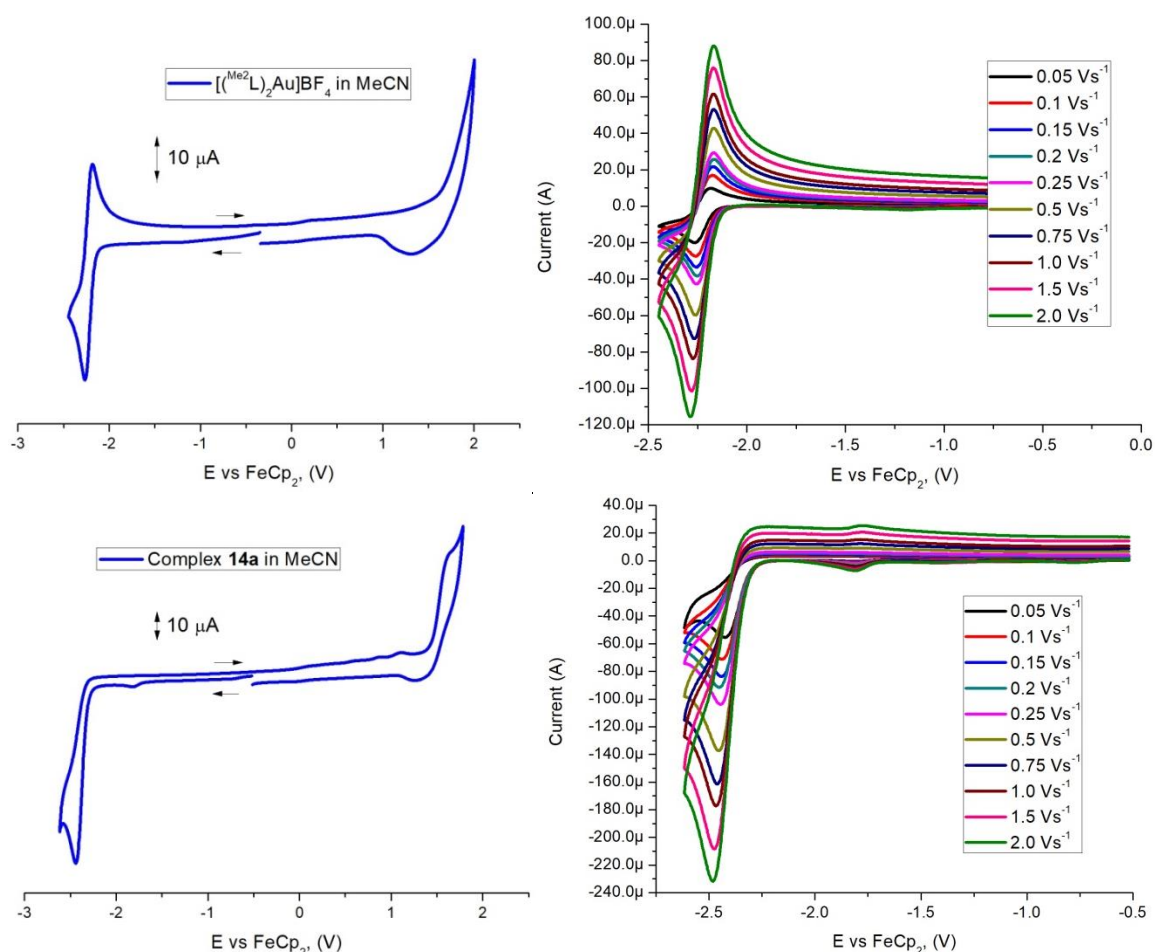
Figure 4. Top Left: full range cyclic voltammogram of homoleptic complex [(\text{Me}^2\text{CAAC})_2\text{Au}]\text{BF}_4 ( 8 ). Top right: Varied scan rate behaviour recorded using a glassy carbon electrode in MeCN solution (1.4 mM) with [\text{Bu}_4\text{N}][\text{PF}_6] as supporting electrolyte (0.13 M). Bottom left: full range cyclic voltammogram of the open-chain carbene complex 14a . Bottom right: Varied scan rate behaviour recorded using a glassy carbon electrode in MeCN solution (2.0 mM) with [\text{Bu}_4\text{N}][\text{PF}_6] as supporting electrolyte (0.13 M).
