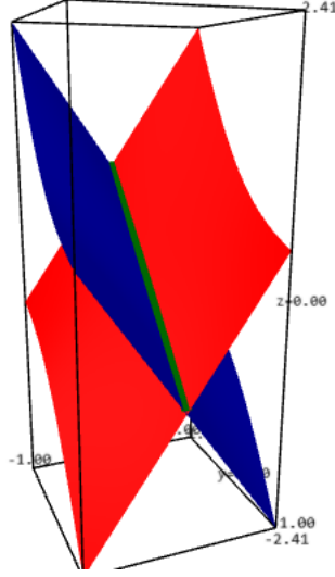
Figure 5: Stratification of \Sigma in the second example.
