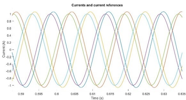
FIG. 6: WINDING CURRENTS AND THEIR REFERENCES WITH A STANDARD PI-CONTROL
