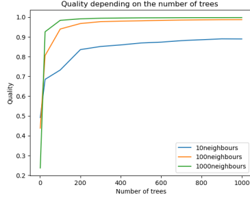
(a) Quality depending on the number of trees
