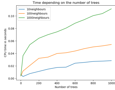
(b) Time depending on the number of trees
