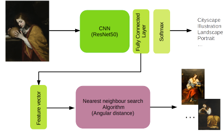
Fig. 1. Schematic representation of our similarity-based image search tool
