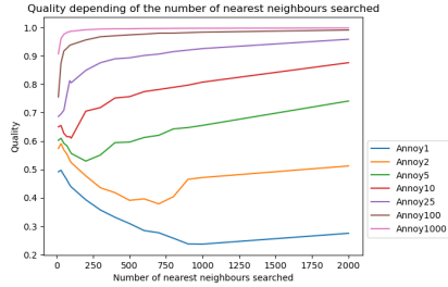
(c) Quality depending on the number of nearest neighbours searched
