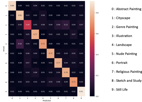
Fig. 3. Confusion matrix on WikiArt test data
