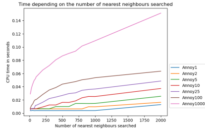
(d) Time depending on the number of nearest neighbours searched
