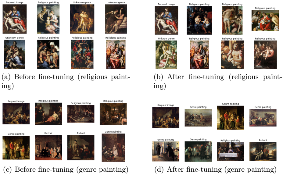
Fig. 4. CBIR performance on an example before and after fine-tuning on a religious painting and on a genre painting
