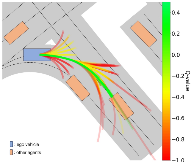
Fig. 1. Visualization of the exploration done by MBAPPE in one planning step. We display the bird-eye-view trajectory pieces in xy coordinates. As the road is turning right, the MCTS explores multiple steering angle and acceleration configurations to correctly take the turn. MBAPPE finally selects the path which maximizes the Q-value (in green).
