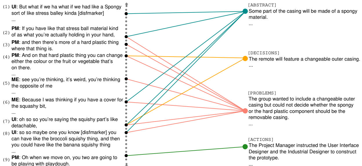
Figure 1: Example (Shang et al., 2020a) of ground truth human annotations from the ES2011c AMI meeting. Successive grey nodes on the left denote utterances recorded in the transcript, the black nodes correspond to a subset of utterances that annotators judged important (summary-worthy). A single sentence from each section of the abstractive summary is shown on the right. The colored arcs link a given sentence from the abstract summary to a single abstractive community; that is, the set of clauses from the extractive summary that is summarized by the sentence from the abstractive summary.
