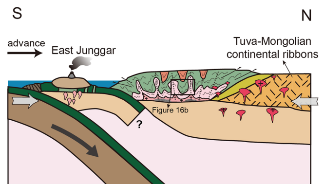
Figure 16. Tectonic sketches correlating Cambrian to Carboniferous tectono-thermal evolution of the Altaï accretionary wedge with alternating advancing and retreating of subduction. (a) Cambrian-Middle Ordovician subduction retreat gave rise to the formation of the Ikh-Mongol Arc and a turbidite basin (future Altaï wedge); (b) Late Ordovician-Early Silurian subduction advance caused thickening and Barrovian metamorphism in the Altaï wedge sequence; (c) Late Silurian-Middle Devonian subduction retreat was responsible for crustal extension in the Altaï and migration of arc fronts into the East Junggar; and (d) Middle Devonian-Early Carboniferous subduction advance generated crustal-scale D2 folding.
