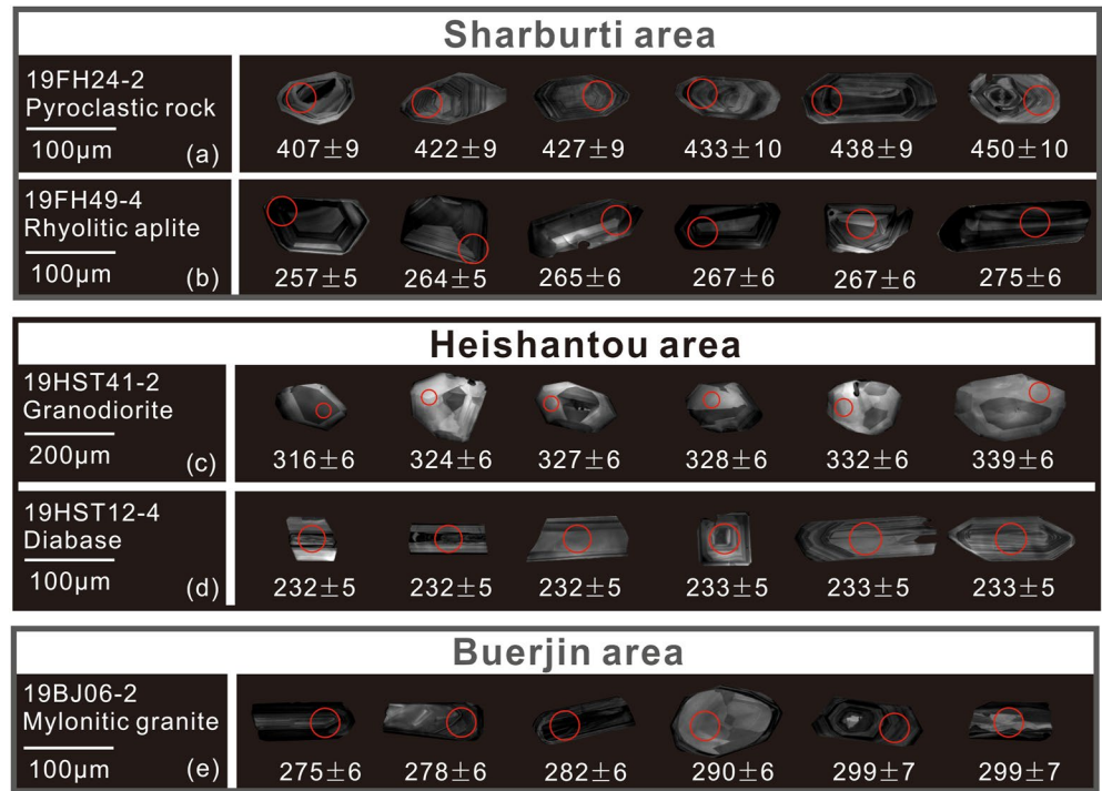
Figure 11. The CL images of zircons from studied samples.
