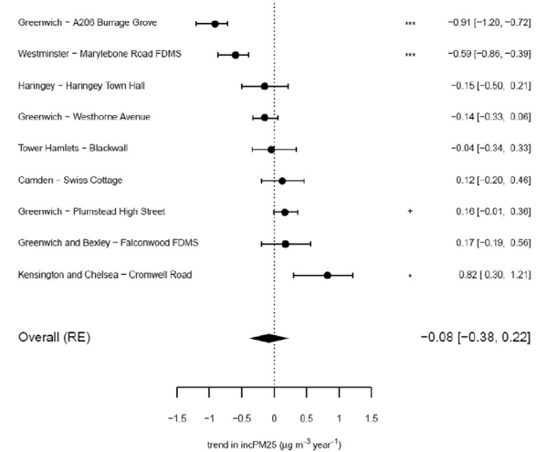
Fig. 4. Forest plots for the trends in roadside increments in NO 2 (incNO 2 ), PM 10 (incPM 10 ), and PM 2.5 (incPM 2.5 ) for Paris and London for 2010–16.
