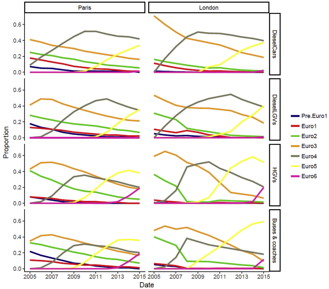
Fig. 2. Distribution of Euro classes for diesel vehicles (cars, LGVs, HGVs and buses & coaches) for Paris and London.
