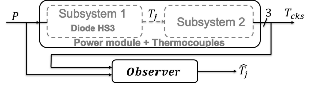
Fig. 11. Closed-loop junction temperature estimation representation: observer design using diode HS3 dissipated power and sensors temperature measurements.
