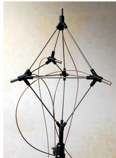
Figure 4: Prototype of an open SMA configuration with 4 B&K© 4958 microphones in a tetrahedral arrangement plus a fifth microphone pointing at the sphere center.
