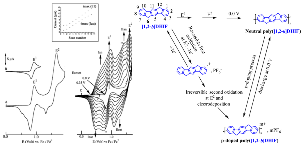
Fig. 3 Cyclic voltammety in the presence of [1,2- b ]DHIF ( 2 \times 10^{-3} M) (A–C) in \text{CH}_2\text{Cl}_2 ( \text{Bu}_4\text{NPF}_6 0.2 M); working electrode: Pt disk diameter 1 mm; sweep-rate 100 \text{ mV s}^{-1} . The potential limit was of 0.0 to 1.75 V in A; 0.0 to 1.0 V in B; -0.2 to 1.73 V in C. The current scale S is equal to 2 in (A) and to 4 in (B) and in (C). The inset reports the i_{\text{max}} at E_1^1 and -i_{\text{max}} at I_{\text{cat}} vs. the scan number. Adapted from ref. 48 with permission from the Royal Society of Chemistry.
