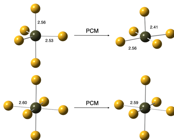
Fig. 1 Representations of the molecular geometries of the bare [\text{PoCl}_5]^- and [\text{PoCl}_6]^{2-} complexes in the gas phase (left) and under the influence of the polarisable continuum model (right). Colour code: polonium (dark green), chlorine (yellow).
