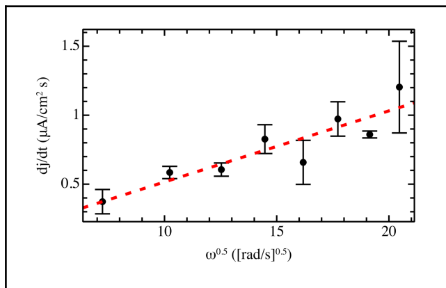
Figure 2: slope of the initial linear increase in current density (the slope of the red dotted line in figure 1) as a function of the square root of the electrode rotation rate. Conditions as in figure 1. The error bars represent the standard deviation across two experiments except for 3000 rpm (3).
