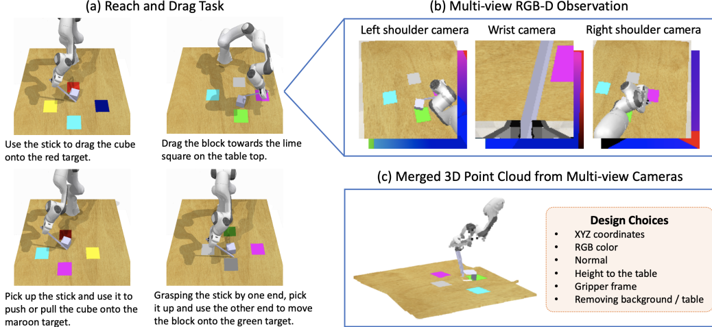
Figure 1: (a): Variations of the “Reach and Drag” task in RLBench [19], with different target colors per variation. (b): Although different views are complementary to represent the scene, they are not explicitly aligned with each other. (c) Merging multi-view cameras to construct a unified point cloud in 3D space. Design options of the point cloud input are carefully investigated in this work.
